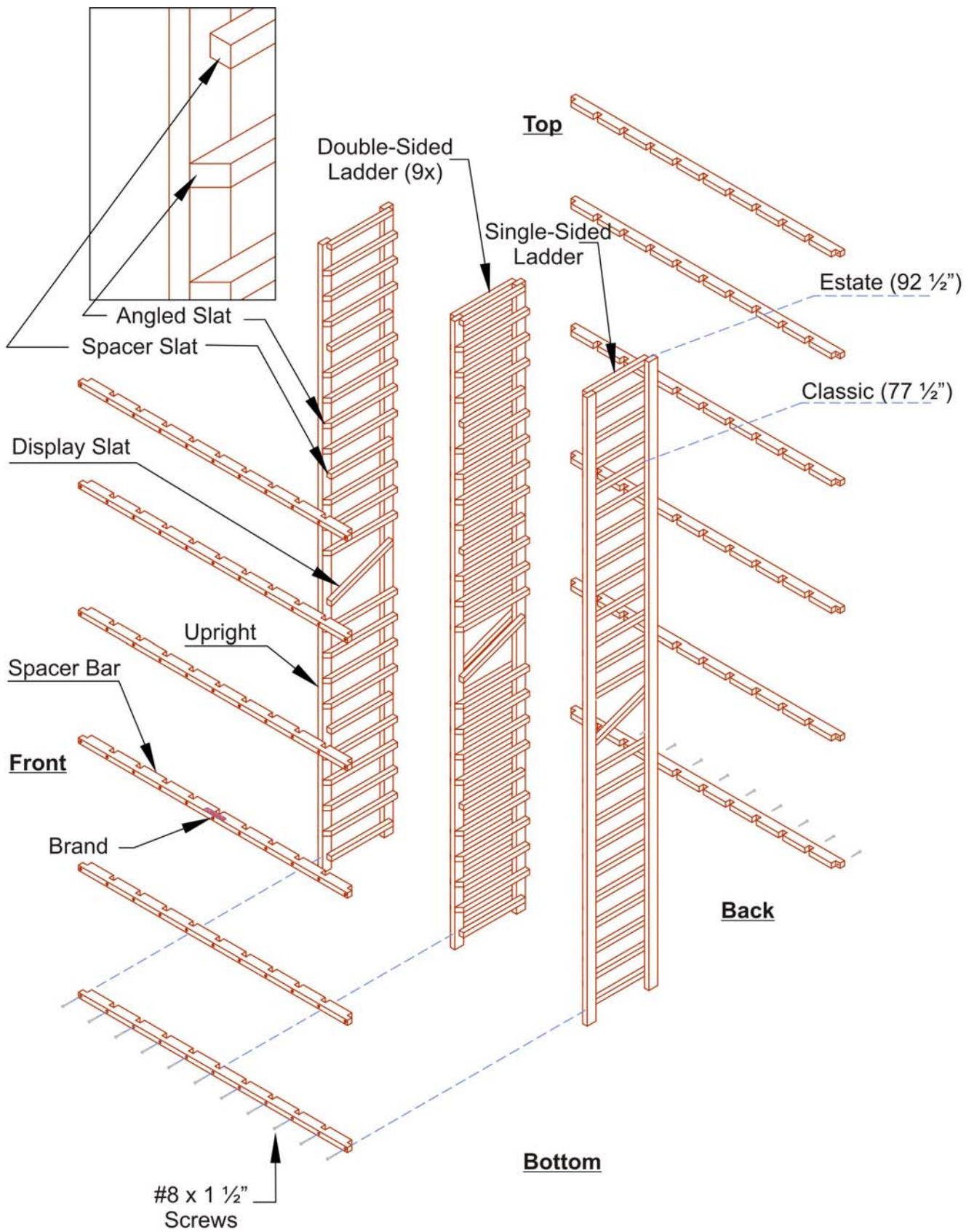
Exploded View (10 Column Rack Shown)
