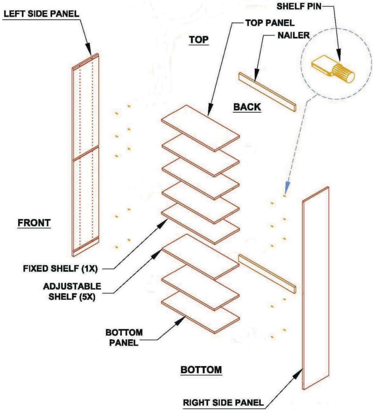
Exploded View
