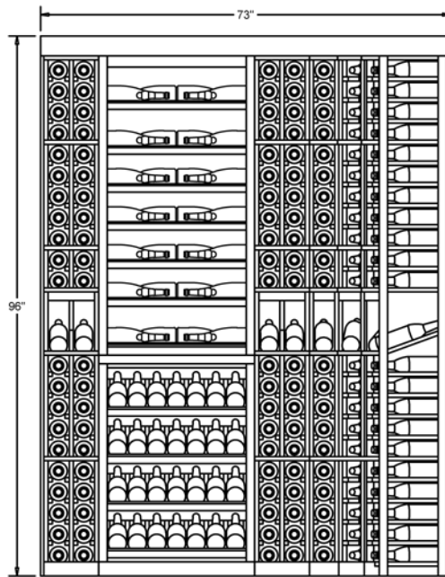
ELEVATION -A-
