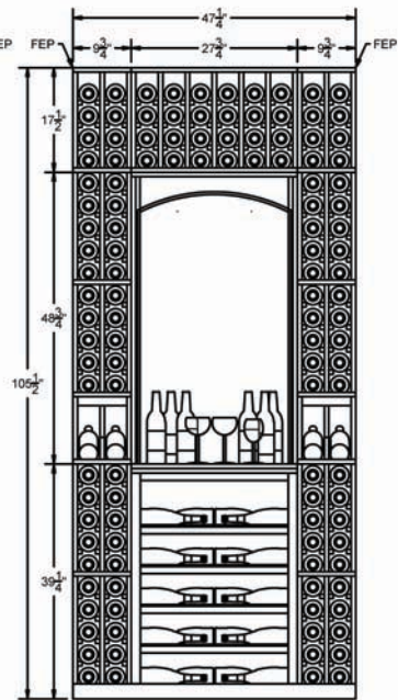
ELEVATION -B-
